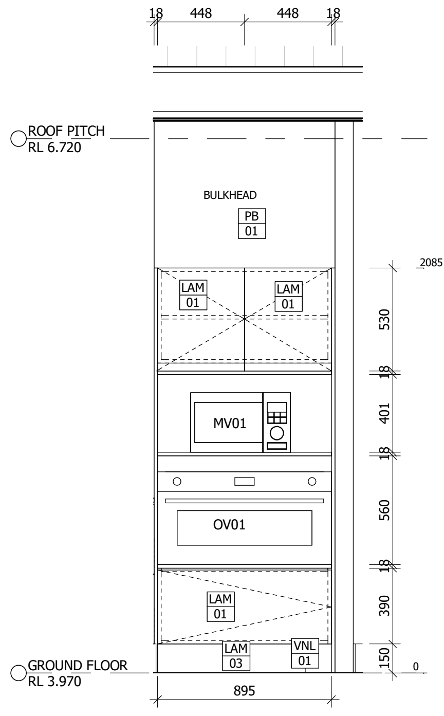
2 J01 - ELEVATION 2 - KITCHEN A4501/ 1 : 20
