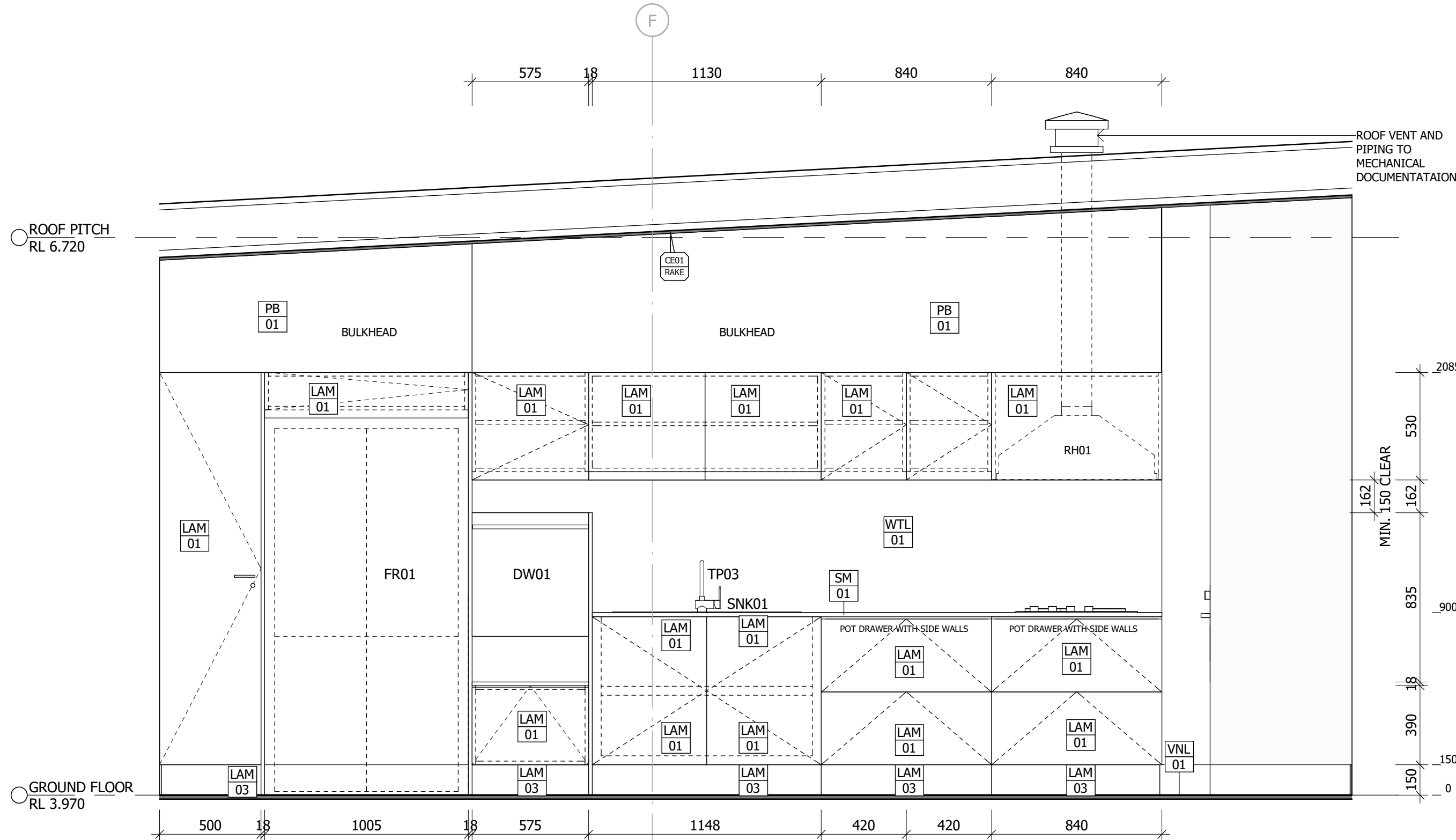
1 J01 - ELEVATION 1 - KITCHEN A4501/ 1 : 20
