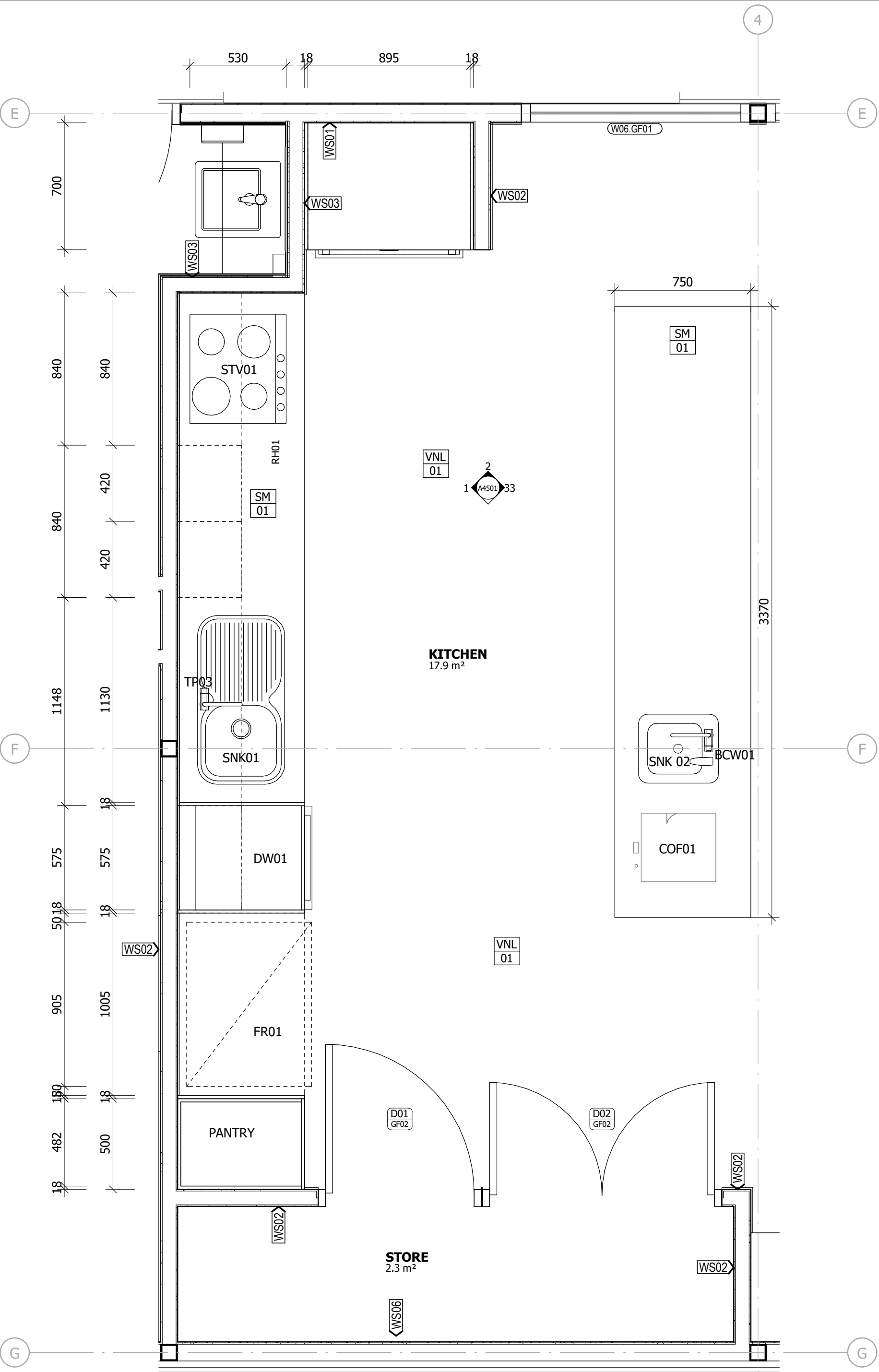
3 GA PLAN - J01 - KITCHEN A2001/ 1 : 20
